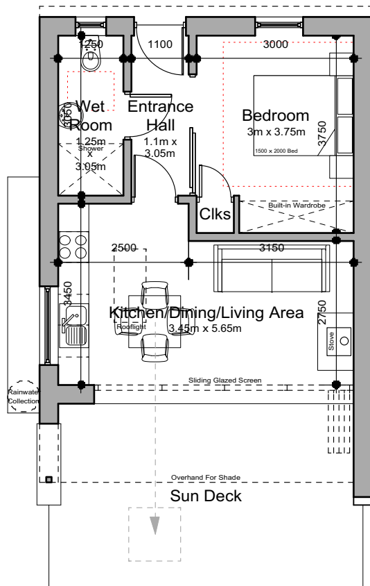
Housetype E Floor Plan (Approx 37.7m 2 ) Scale 1:100
