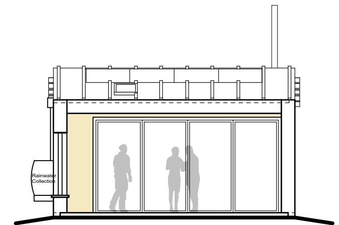
Housetype E South Elevation Scale 1:100
