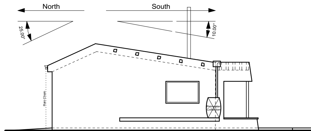
Housetype E West Elevation Scale 1:100
