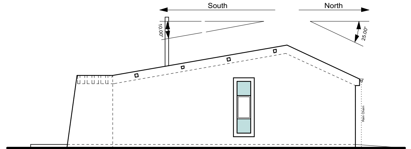
Housetype D East Elevation Scale 1:100
