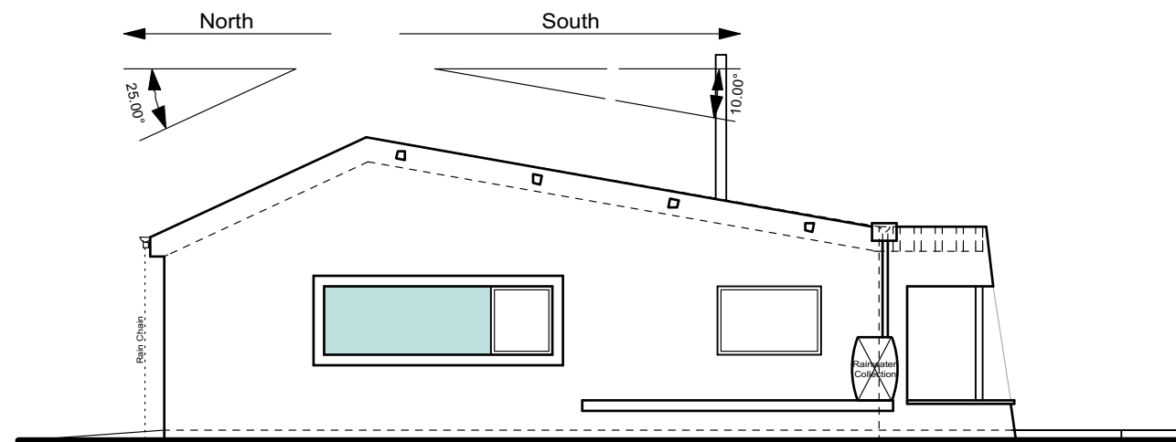
Housetype D West Elevation Scale 1:100
