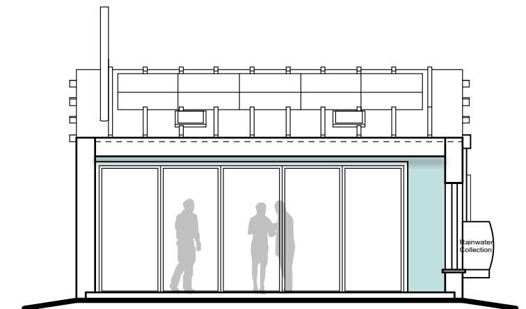
Housetype D South Elevation Scale 1:100
