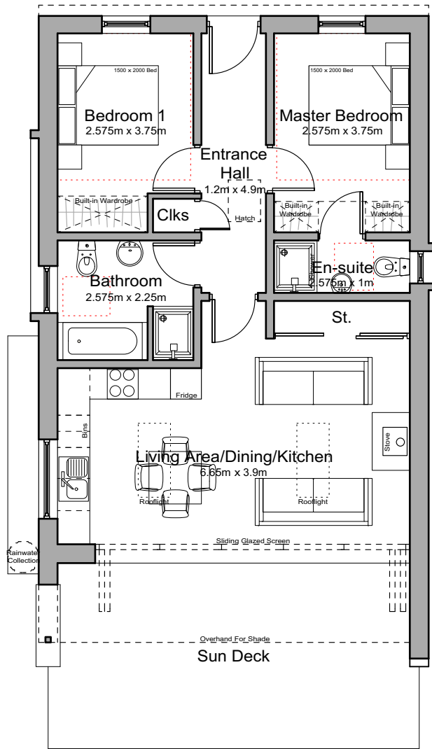
Housetype D Floor Plan (Approx 64.3m 2 ) Scale 1:100
